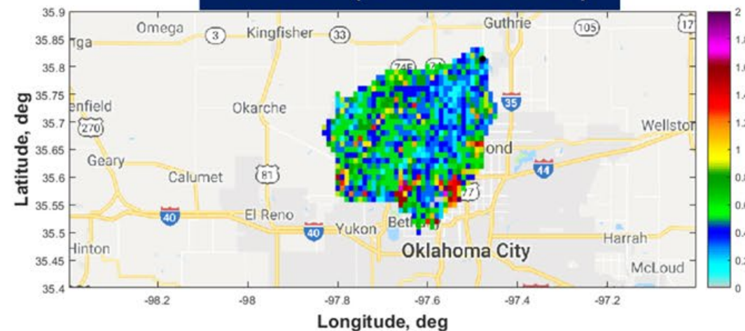
KTLX (5-min/1-km)
