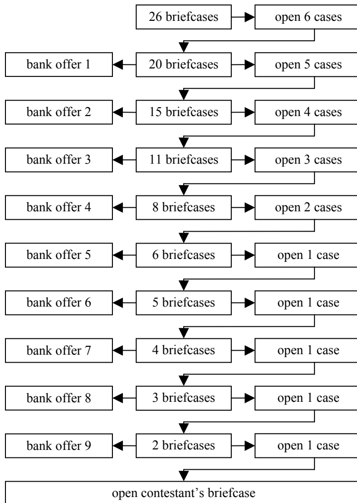
Figure 1: Flow Chart of the Main Game. In each round, the finalist chooses a number of briefcases to be opened, each giving new information about the unknown prize in the contestant’s own briefcase. After the prizes in the chosen briefcases are revealed, a “bank offer” is presented to the finalist. If the contestant accepts the offer (“Deal”), she walks away with the amount offered and the game ends; if the contestant rejects the offer (“No Deal”), play continues and she enters the next round. If the contestant decides “No Deal” in the ninth round, she receives the prize in her own briefcase. The flow chart applies to the Dutch and US editions and the second German series. The first German series involves one fewer game round and starts with 20 briefcases.
