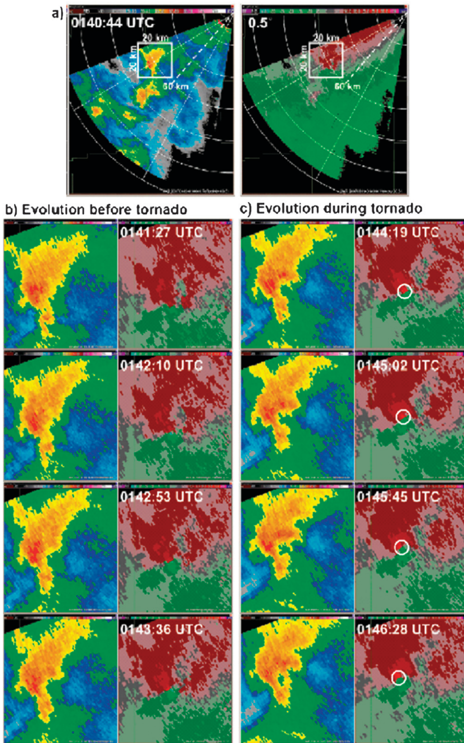
FIG. 6. (a) A 60° sector scan of 0.5°-elevation (left) reflectivity (dBZ) and (right) velocity ( m s^{-1} ) fields at 0140:44 UTC 19 Aug 2007. Range rings are in 20-km increments. The white box denotes the location and scale of the storm whose evolution at the 0.5° tilt is shown (b) prior to and (c) during an EF1-rated tornado. The white circles enclose the tornadic vortex signature.
