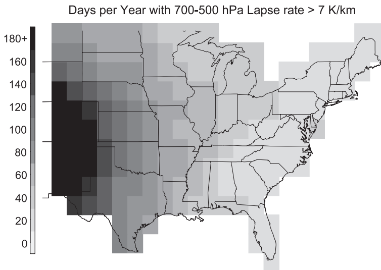
Fig. 7. Same as Fig. 6, except for 700–500 hPa lapse rates exceeding 7 \text{ K km}^{-1} .
