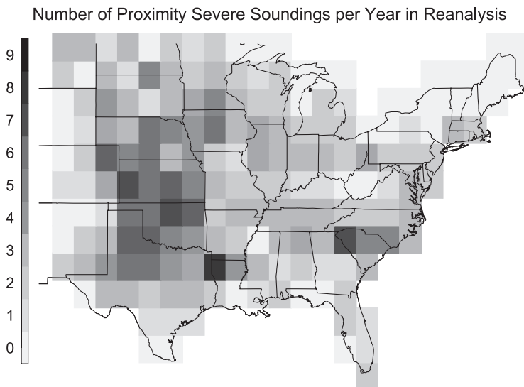
Fig. 12. Same as Fig. 6, except for number of reanalysis soundings associated with significant severe thunderstorms.
