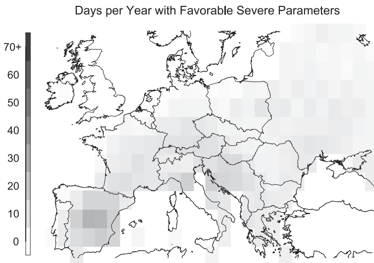
Fig. 15. Same as Fig. 11, except for European region.
