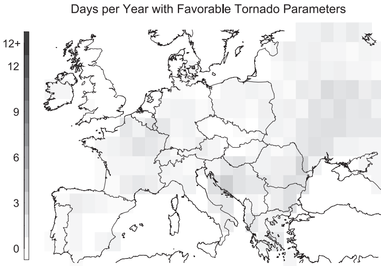
Fig. 16. Same as Fig. 12, except for European region.
