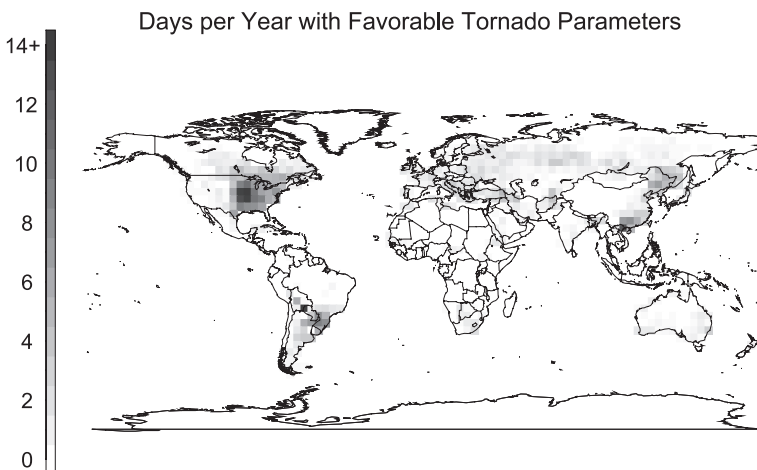
Fig. 18. Same as Fig. 17, except for tornadic parameters.
