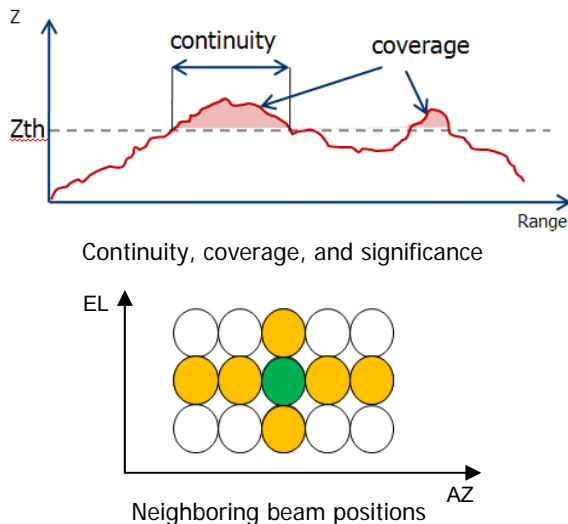
Fig. 1. Second and third criteria for active beam determination in ADAPTS. (top) Depiction of continuity, coverage, and significance conditions based on a range profile of reflectivity. (bottom) Depiction of neighboring beam positions (orange) for an active beam position based on first and/or second criteria (green).
