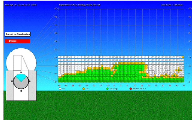
Fig. 2. Depiction of ADAPTS’ real-time performance at the NWRP PAR user interface. Beam positions on an azimuth-by-elevation plane are color-coded as follows: white beam positions are inactive, green beam positions are active based on elevation and coverage criteria, and orange beam positions are active based on the neighborhood criterion.
