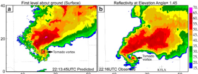
A Warn-on-Forecast model (left) predicts a tornado will form in 33 minutes. (Right) Actual radar observation showing the tornado did form. Image provided by Warn-on-Forecast partners at the Center for the Analysis and Prediction of Storms.
